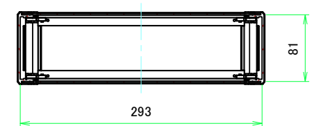
C-C (1:4.5)
