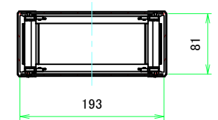
C-C (1:5)
