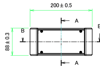
A view
