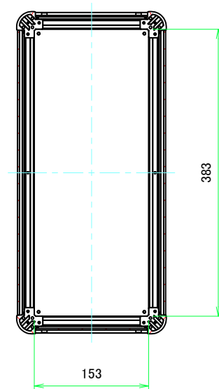
B-B (1:5)
