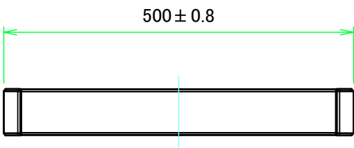
C view
