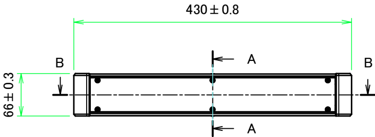
A view
