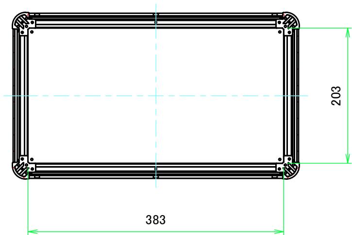
B-B ( 1:5.5 )
