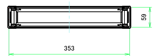
C-C ( 1:5.5 )
