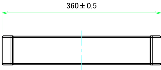
C view
