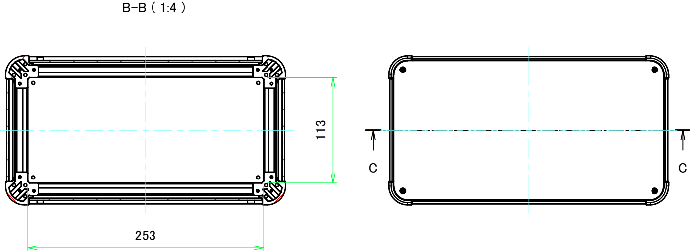
E view
