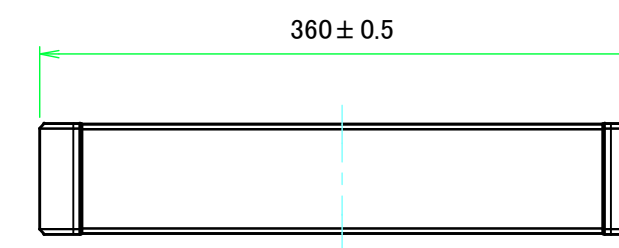
C view
