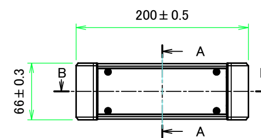
A view
