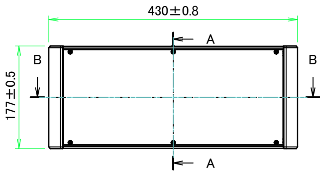
A view
