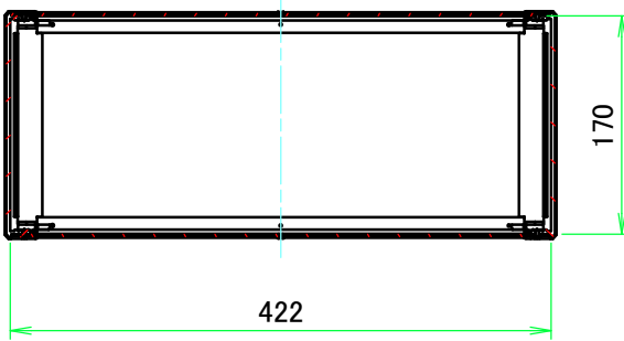
C-C ( 1 :6.5 )
