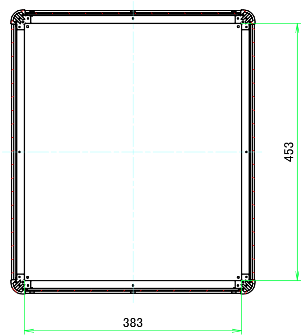
B-B ( 1 :6.5 )
