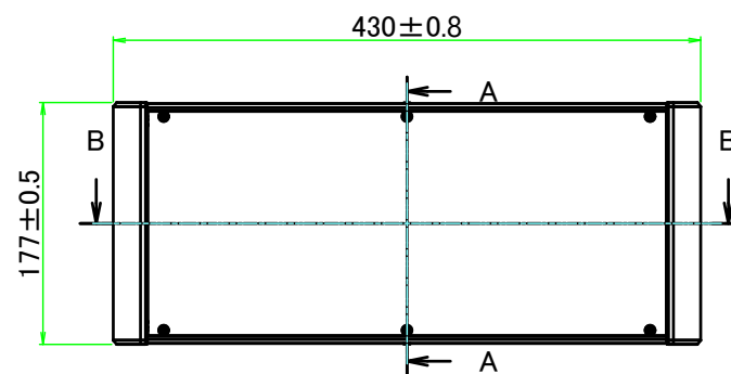
A view
