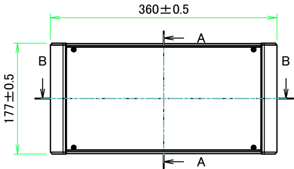
A view
