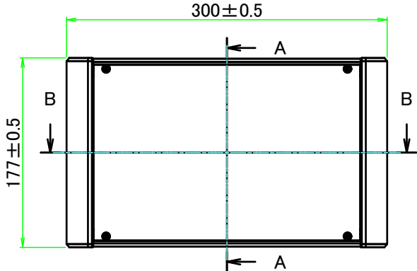
A view
