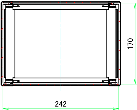
C-C ( 1 :4.5 )
