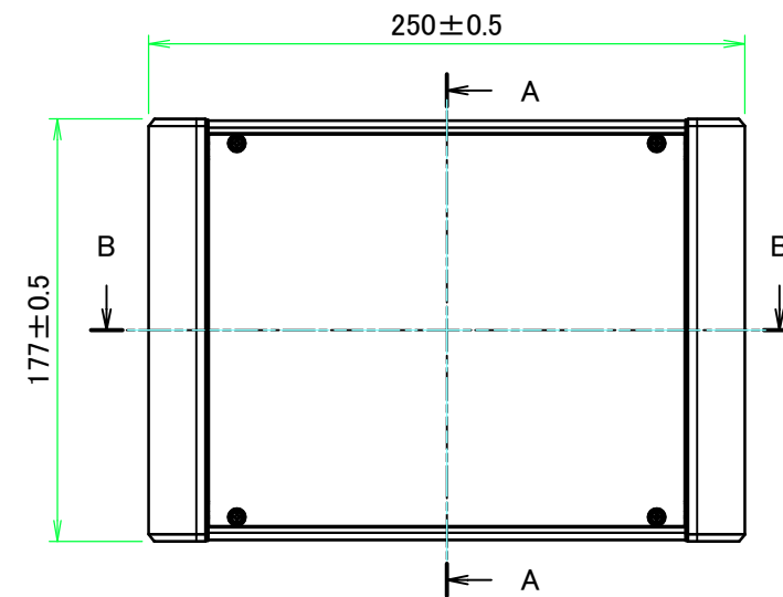
A view
