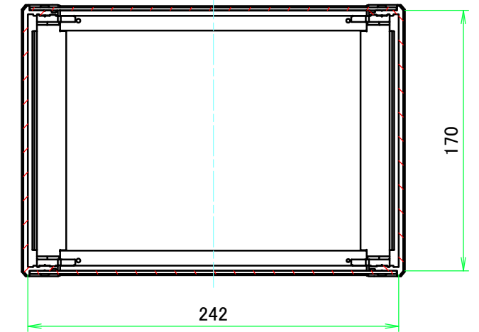
C-C ( 1 :3.5 )
