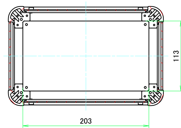
B-B ( 1 :3.5 )
