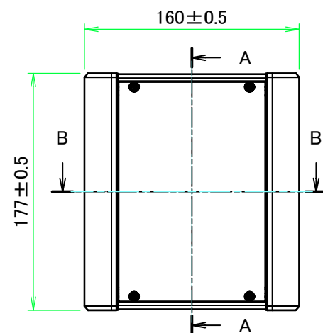
A view
