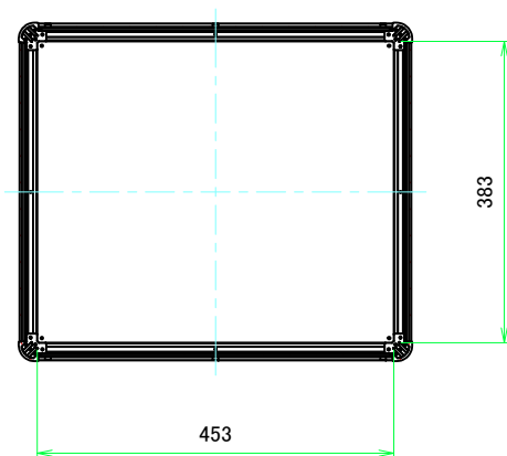
B-B (1:7.5)
