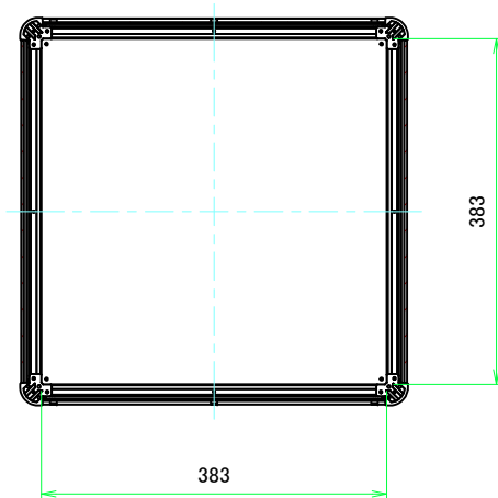
D view
