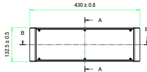
F view
