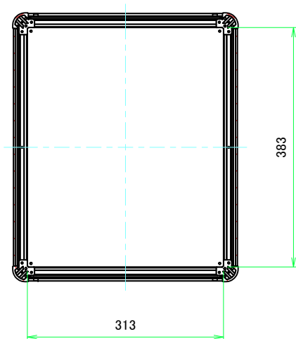
B-B (1:6)
