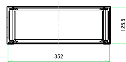
C-C (1:5.5)
