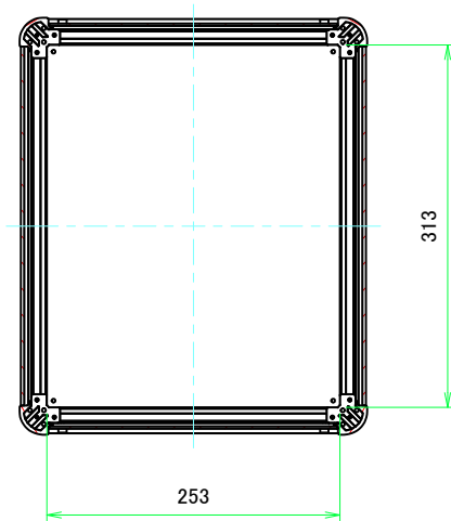
B-B (1:5)
