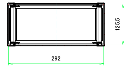
C-C (1:5)
