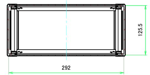
C-C (1:4)
