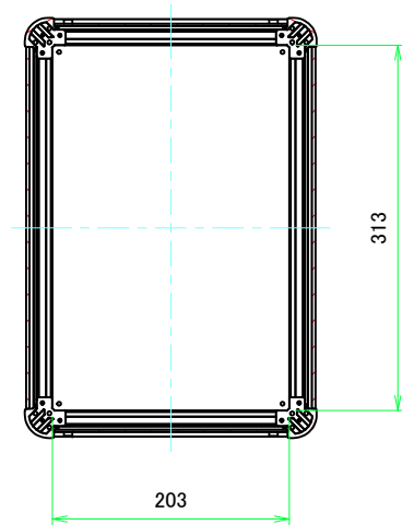
B-B (1:5)
