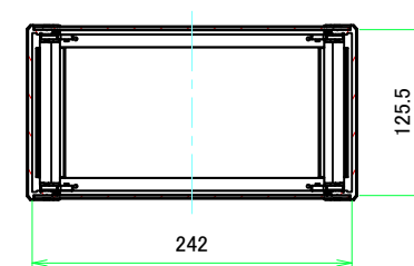
C-C (1:4.5)
