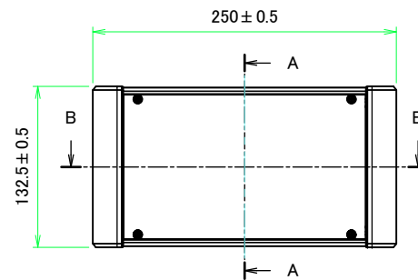
F view
