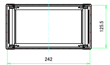
C-C (1:4)
