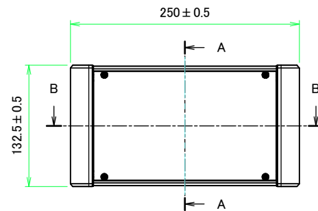
A view
