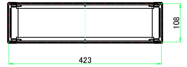
C-C ( 1 :6.5 )
