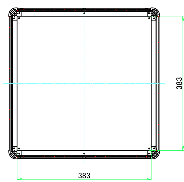
B-B ( 1 :6.5 )
