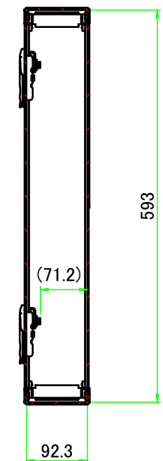
B-B (1:8)
