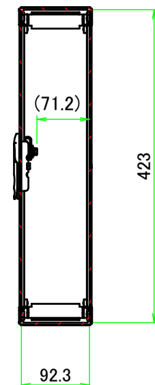
B-B (1:7)
