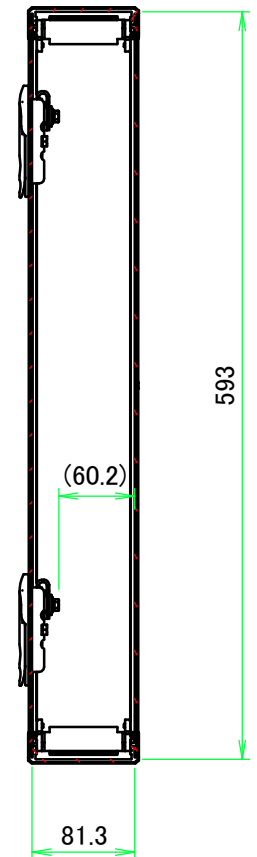
B-B (1:6)
