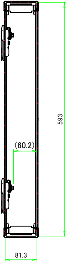
B-B (1:6)
