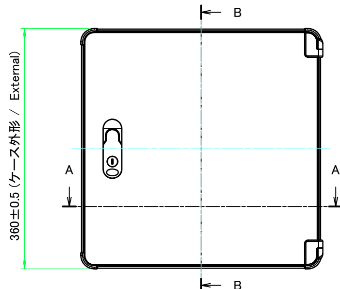
A view
