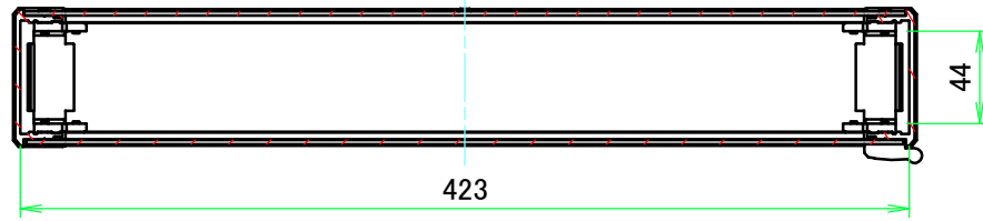
E view
