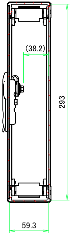
B-B ( 1 :3.5 )
