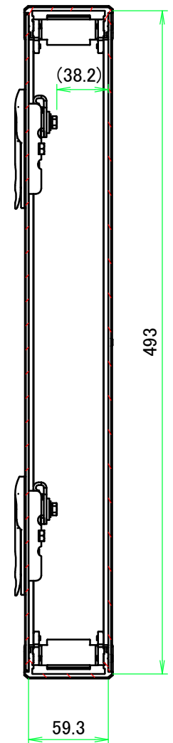
B-B (1:4)
