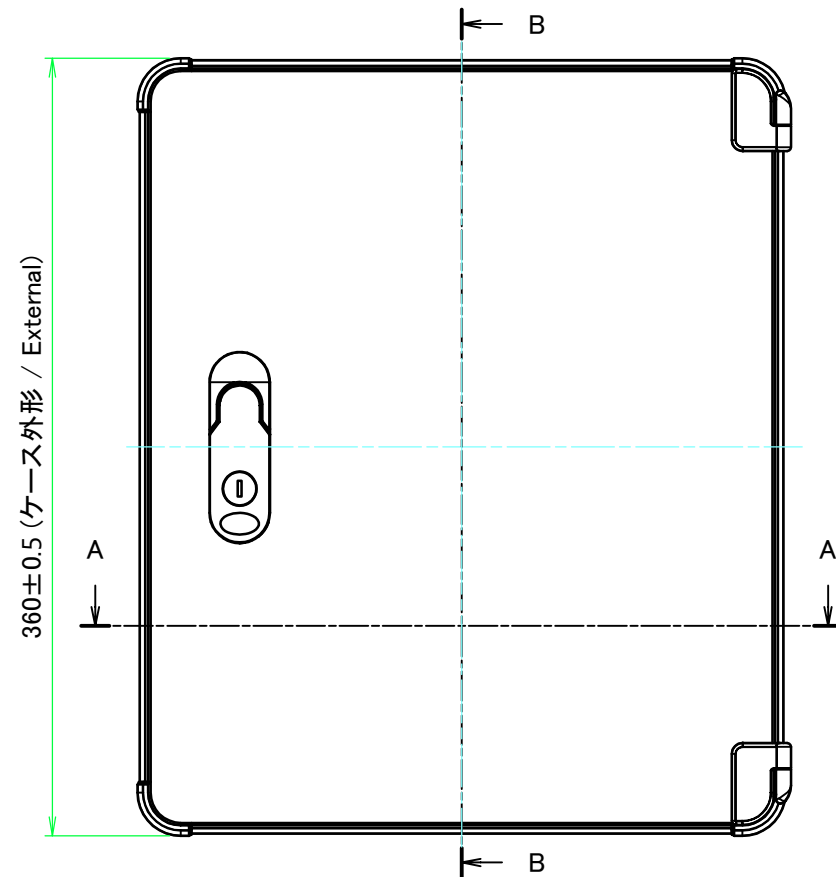
A view
