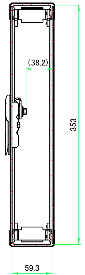
B-B ( 1 :3.5 )
