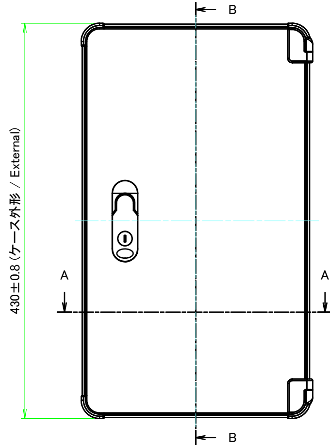
A view
