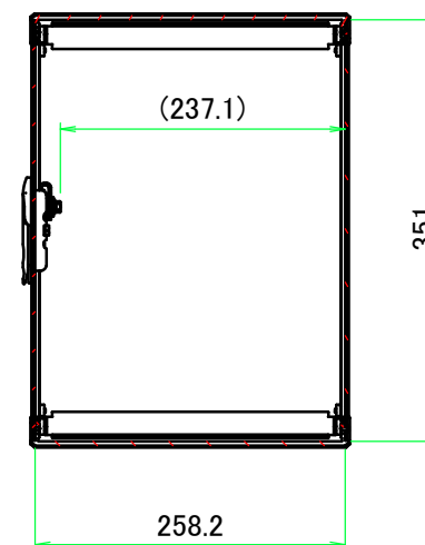
B-B (1:7)
