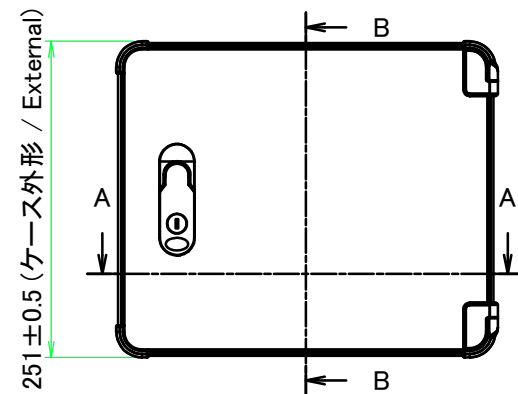
A view
