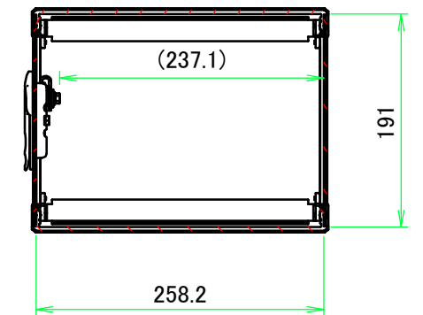
B-B (1:6)
