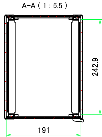
E view
