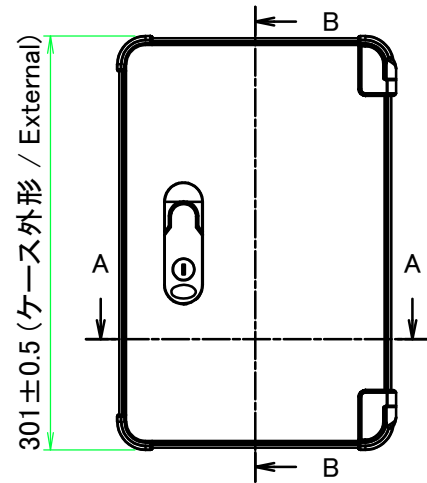
F view
