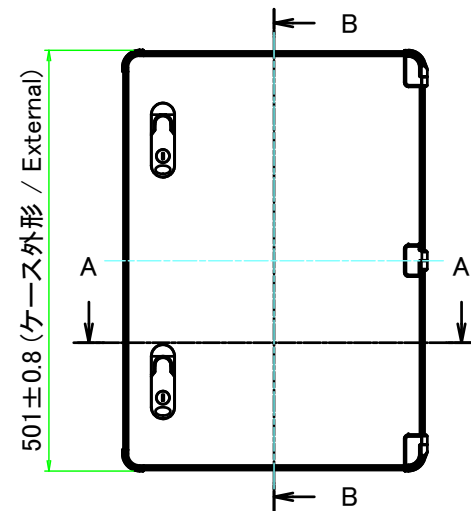
A view
