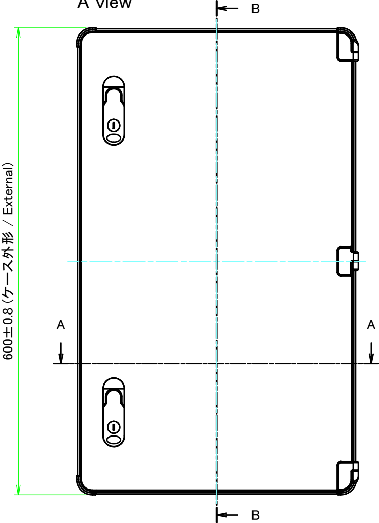
A view
