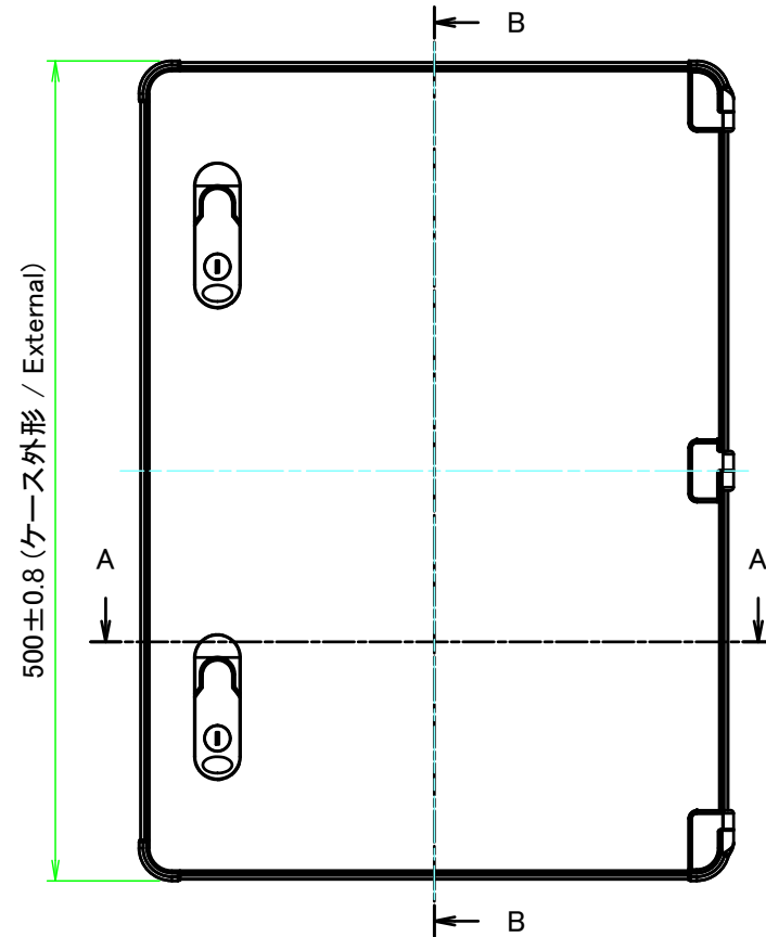
A view
