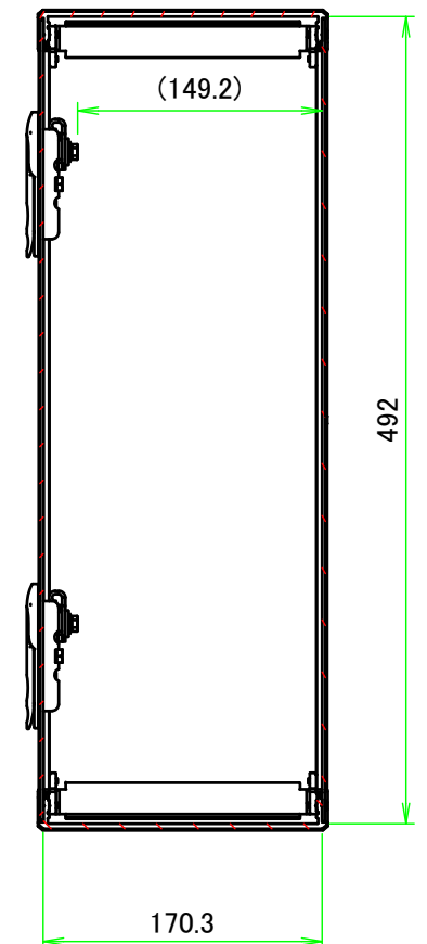
B-B (1:5)
