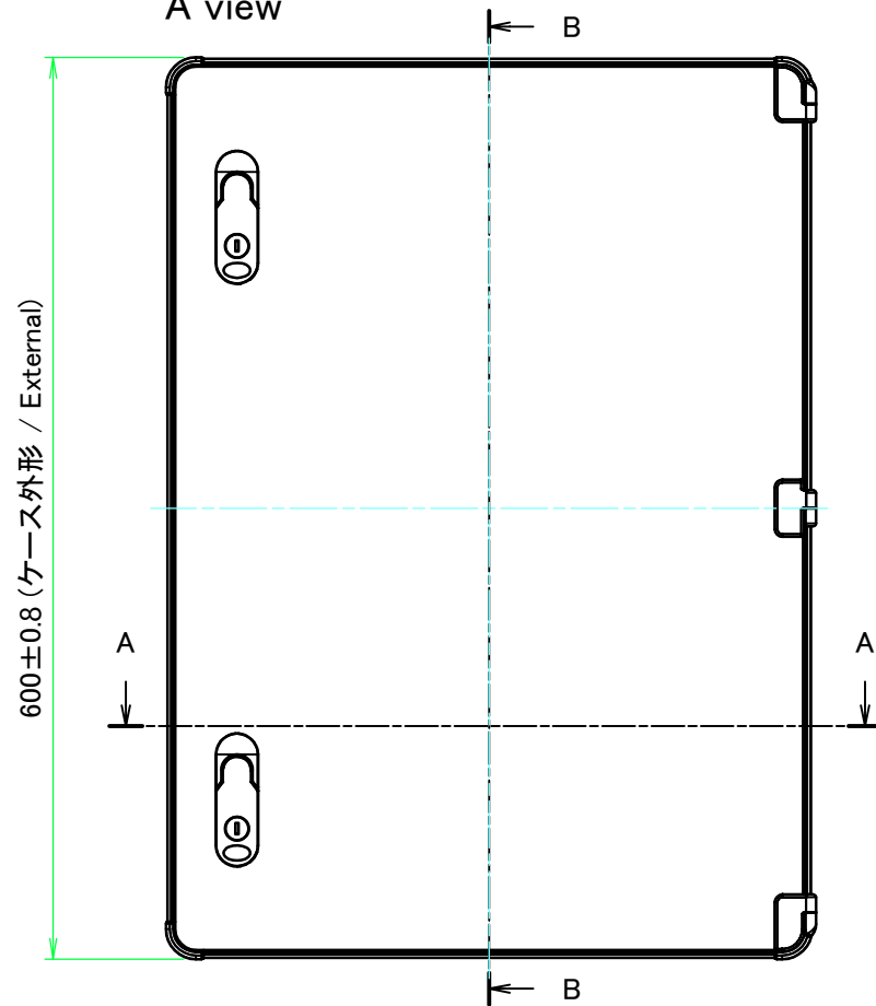
A view
