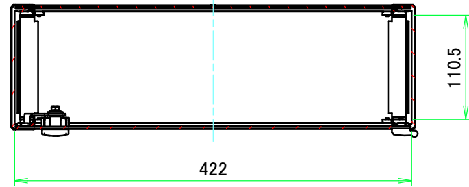
E view
