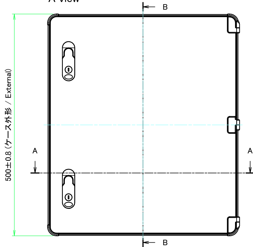
A view
