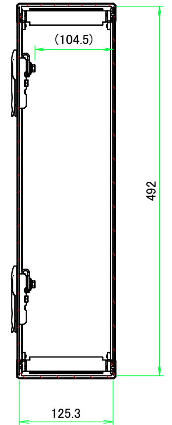
B-B (1:5)
