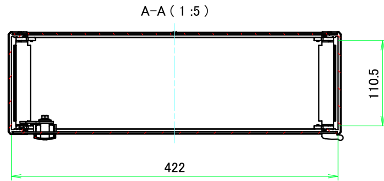
E view
