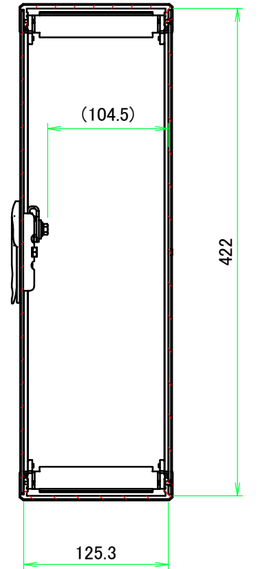
B-B ( 1 :4.5 )
