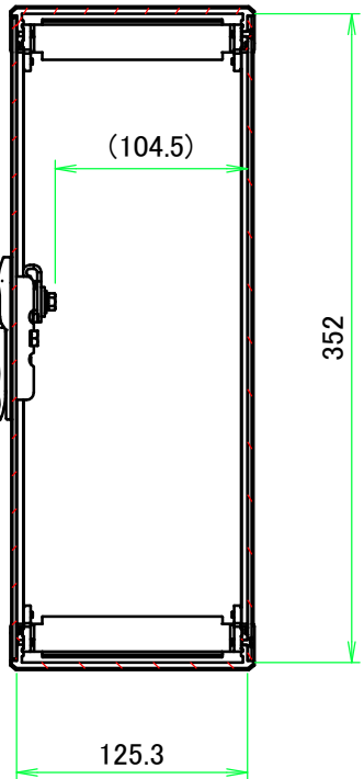
B-B ( 1 :4.5 )
