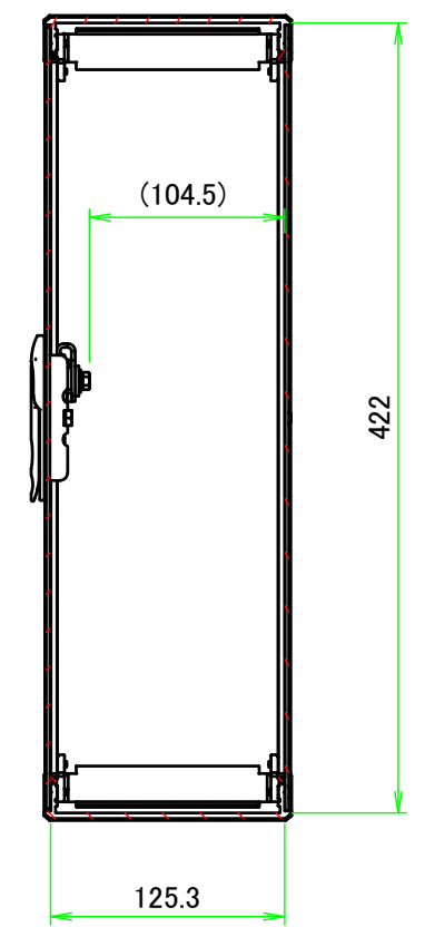
B-B ( 1 :4.5 )
